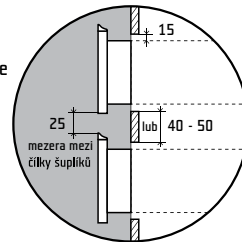
drawing for the handle QE23 (mm)
