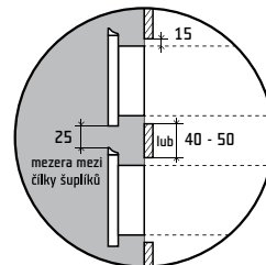
drawing for the handle QE22 (mm)
